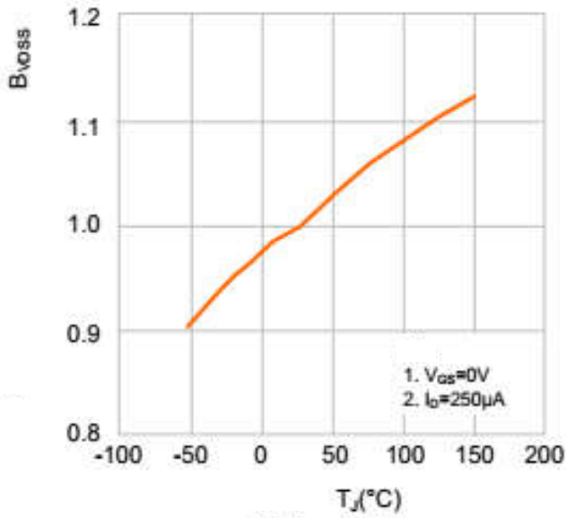
Figure7. Typical Breakdown Voltage vs Junation Temperature
